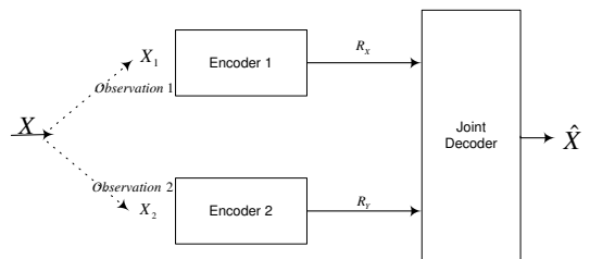
Figure 1: Distributed Source Coding Scheme of the proposed method. Two noisy version of the image are encoded independently and decoded jointly.
