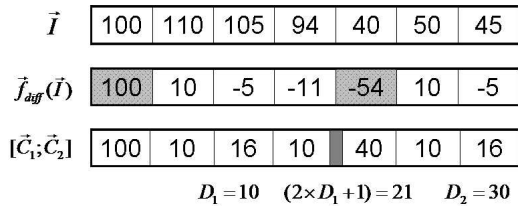
Figure 5: A coset creation example.
